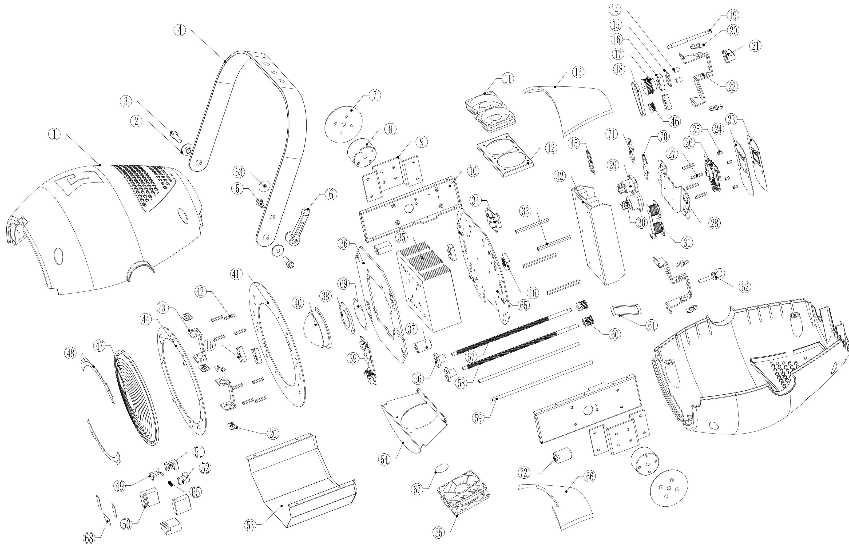
B EXPO200MCW / WW EXPLODED VIEW
