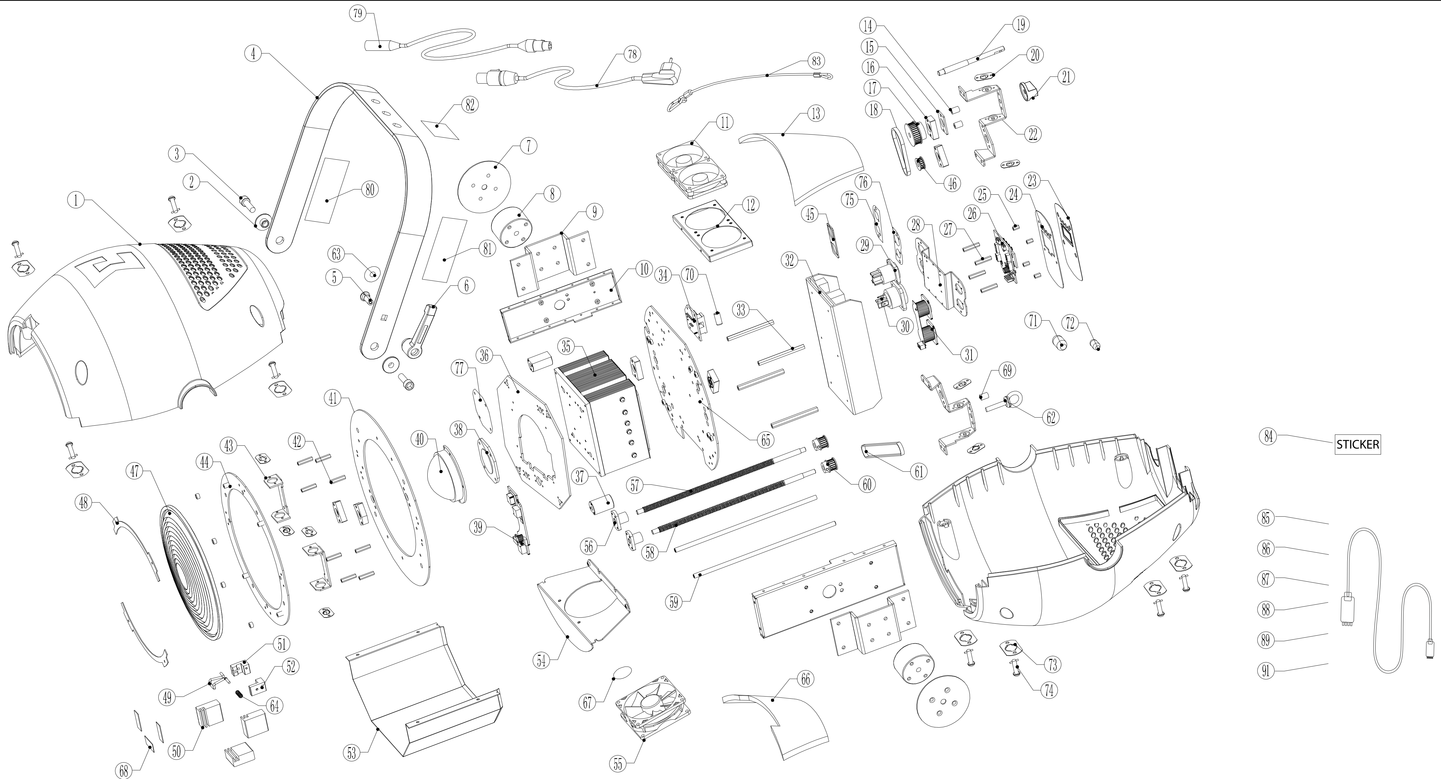
B EXPO350MCW / WW EXPLODED VIEW
